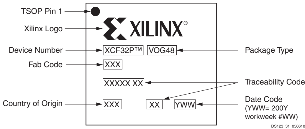
Figure 15: 48-Pin TSOP Marking
