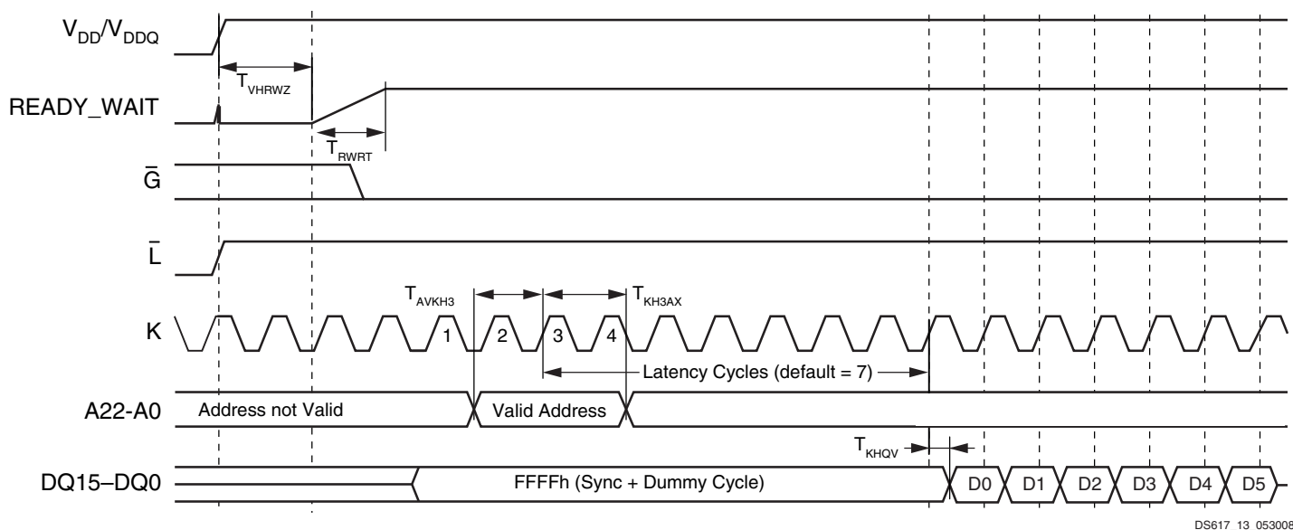
Figure 17: Power-Up Sequence (System with Free-Running Clock)
