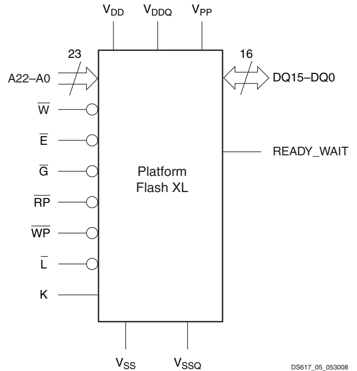
Figure 5: Logic Diagram
