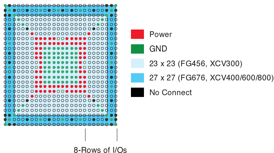
Figure 5-4: Fine Pitch BGA Pin Assignments
