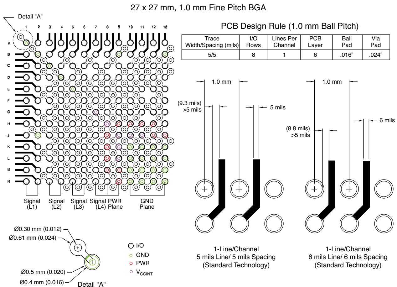
Figure 5-5: FG676 PC Board Layout/Land Pattern
