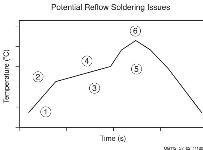
Figure 7-2: Soldering Problems Summary
