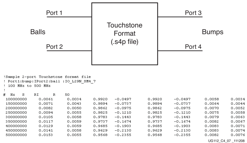
Figure 4-7: 4-port Assignment Convention and Illustration of 2-port Touchstone Format
