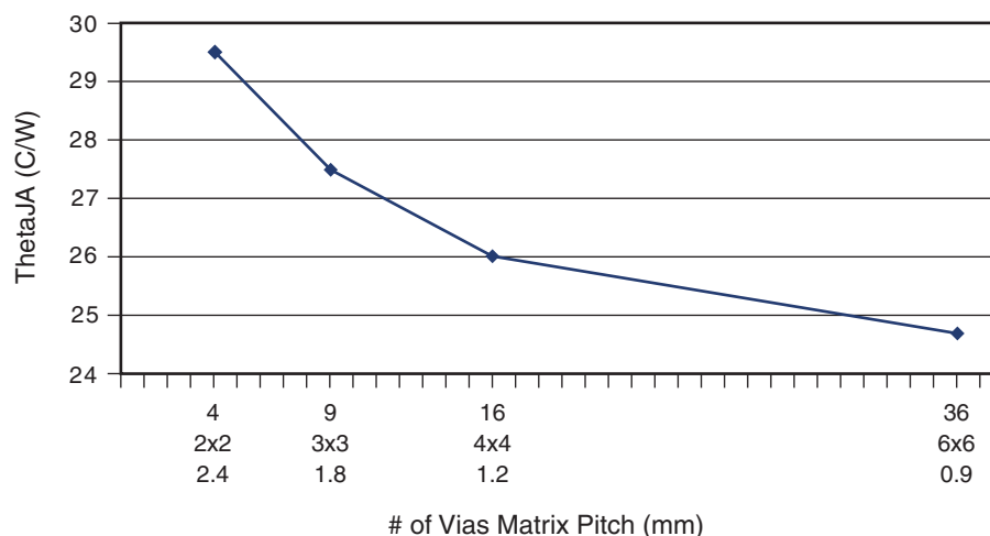
Figure 5-14: \theta_{JA} vs. Number of Vias Graph
