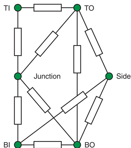
Figure 3-1: Compact Thermal Model Topologies
