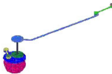
Figure 4-3: Flip Chip Interconnect Chain
