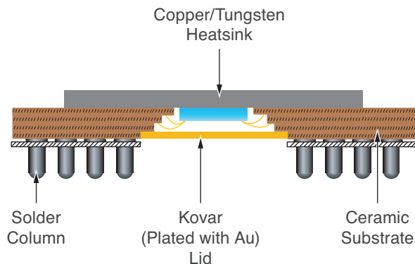
Figure 1-9: CG560 Package
