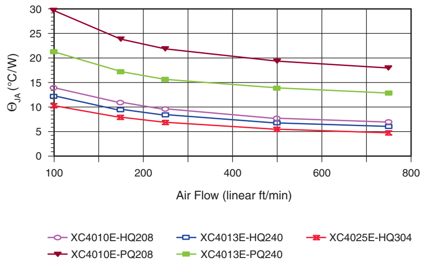
Figure 3-4: Effect of Air Flow on the Thermal Resistance ( \theta_{JA} ) of HQ/PQ Packages
