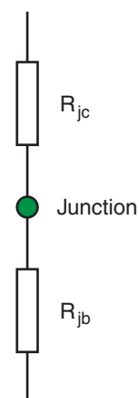
Two-Resistor Model
