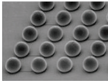
Figure 1-4: Eutectic Bumps
