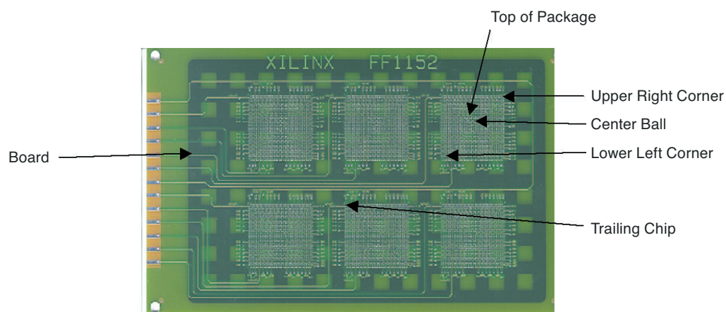
Figure 7-4: Temperature Measurement Locations
