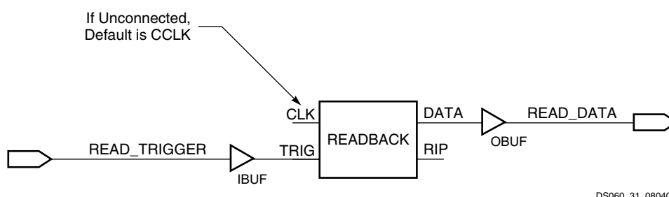
Figure 32: Readback Example
