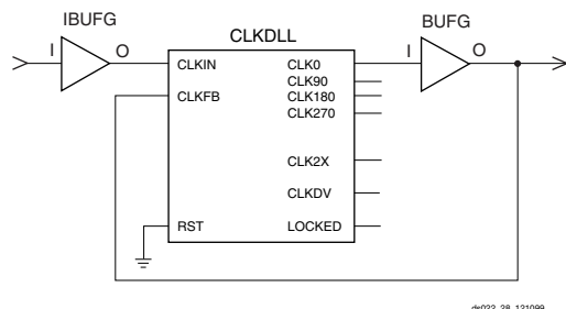
Figure 24: BUFGDLL Schematic
