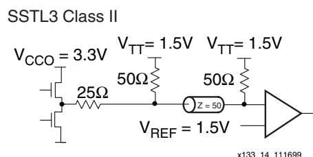
Figure 50: Terminated SSTL3 Class II
