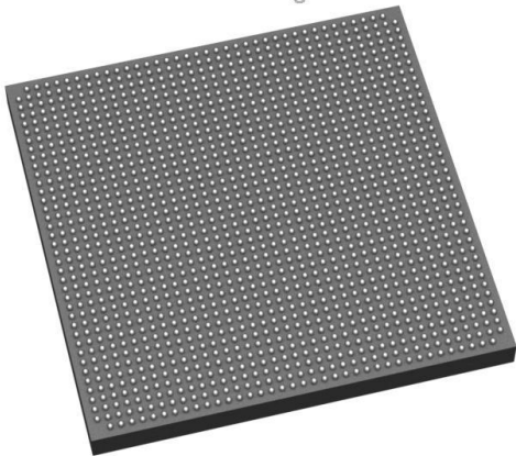
XCZU43DR-2F5VG1517I
