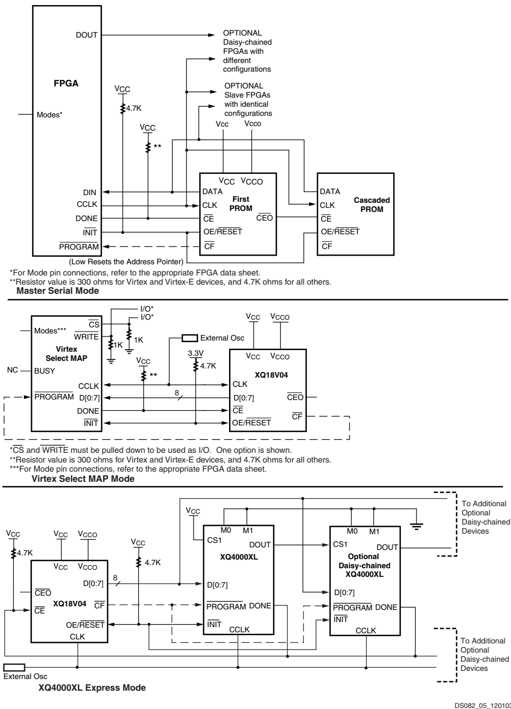
Figure 3: (a) Master Serial Mode (b) Virtex SelectMAP Mode (c) XQ4000XL Express Mode (dotted lines indicate optional connection)
