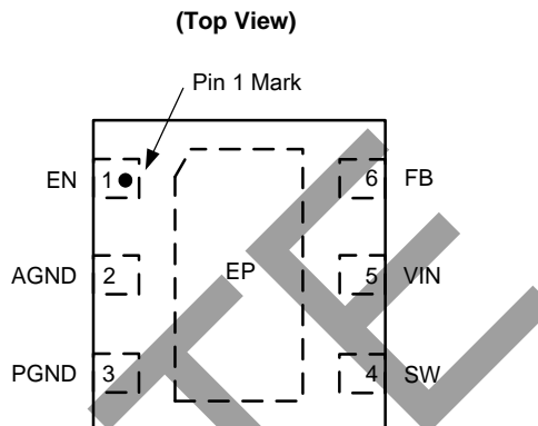
U-DFN1616-6 (Type G)
