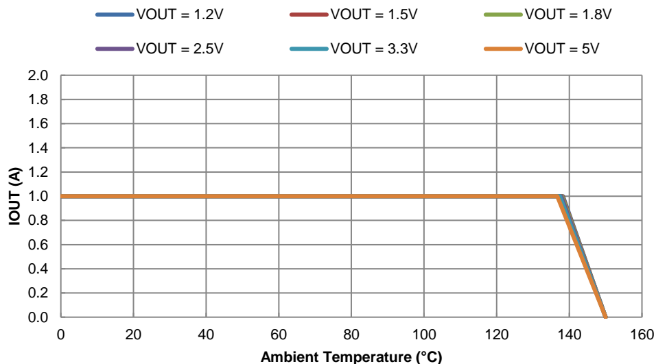
Figure 26. Output Current Derating Curve vs. Ambient Temperature, V_{\text{IN}} = 12\text{V} , f_{\text{sw}} = 500\text{kHz}
