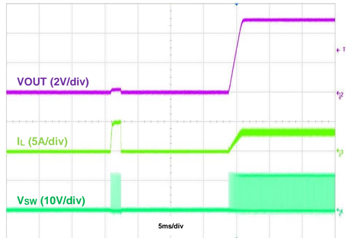
Figure 22. Output Short Recovery, IOU = 3.5A
