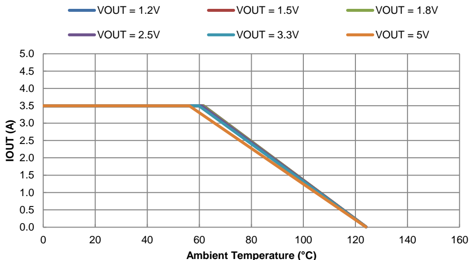
Figure 24. Output Current Derating Curve vs. Ambient Temperature, V_{\text{IN}} = 12\text{V} , f_{\text{sw}} = 500\text{kHz}
