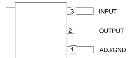
TO252-2
