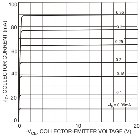
Figure 2 Typical Collector Current vs. Collector-Emitter Voltage
