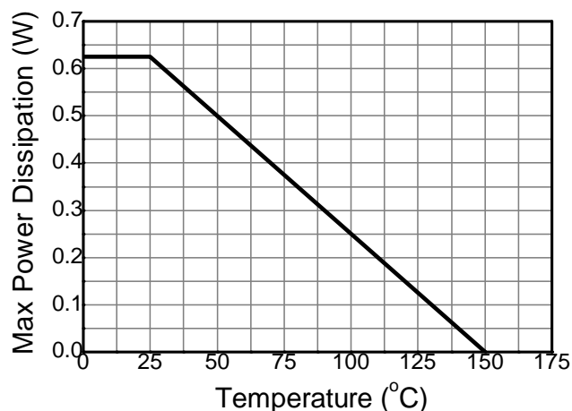
Derating Curve
