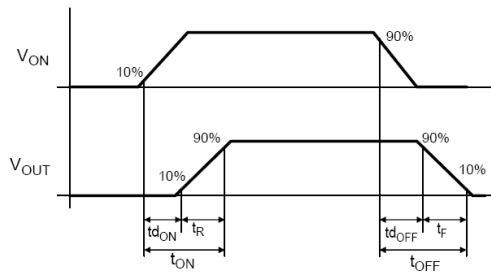
Figure 27. Timing Diagram
