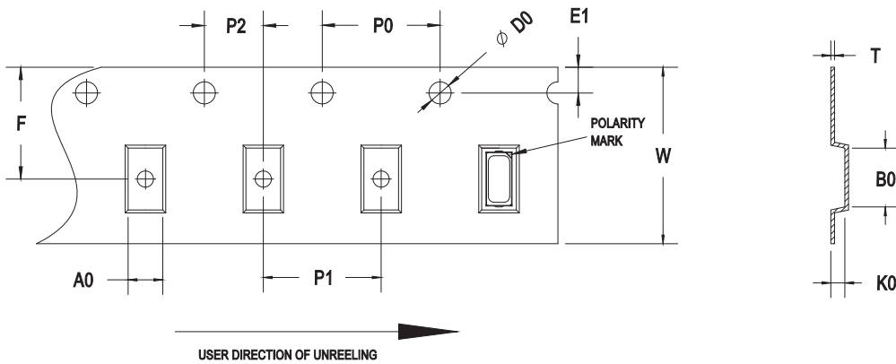
Figure 17: Carrier Tape Dimensions
