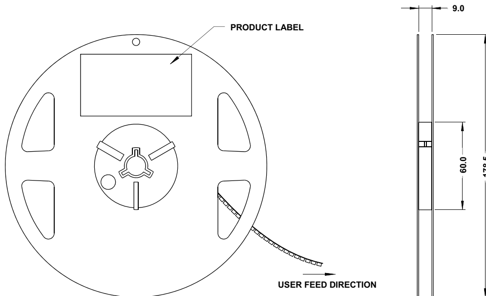
Figure 18: Reel Dimensions
