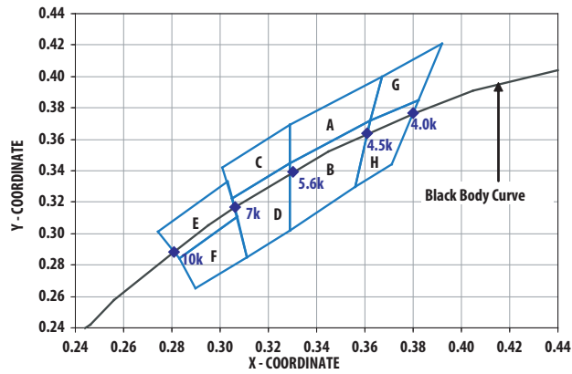
Figure 18. Color bins (Cool White).
