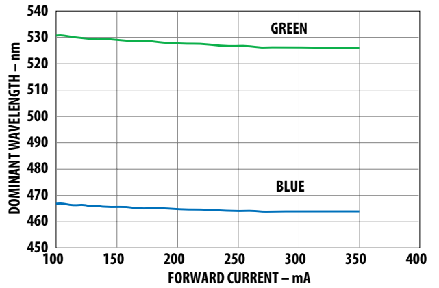
Figure 12. Dominant wavelength vs. forward current - InGaN devices
