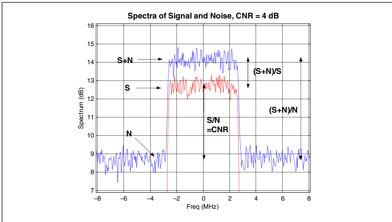
Figure 7: Close-Up View of Signal and Noise As Measured on a Spectrum Analyzer
