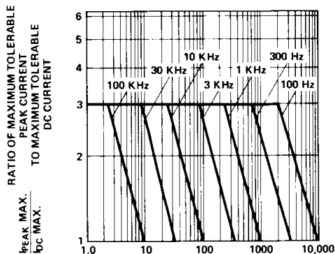
Figure 12: Maximum Tolerable Peak Current vs. Pulse Duration. (I DC MAX as per MAX ratings)
