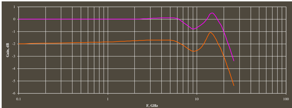
Fig. 4. THA Gain at Max and Min gainctrl Values vs. Data Frequency
