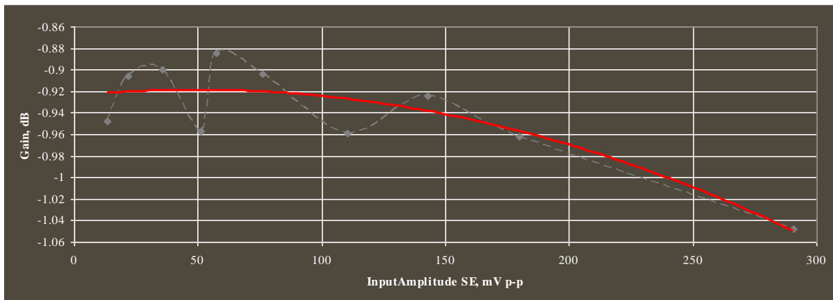
Fig. 6. THA Gain vs. Input Data Amplitude at Medium State of gainctrl
