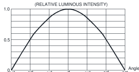
FIG.6 FAR FIELD PATTERN
