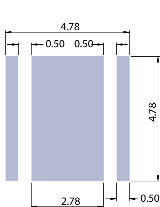
Recommended PCB Footprint
