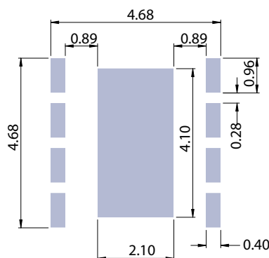
Recommended Solder Stencil*
