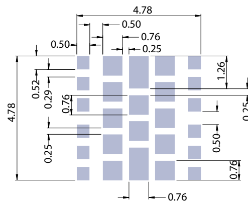
Optional Solder Stencil*
